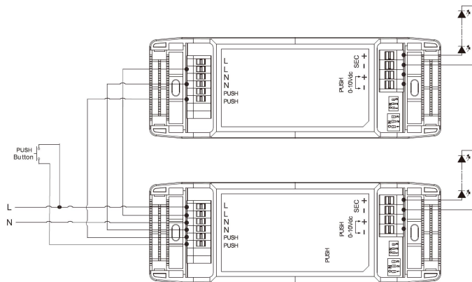
Fig. A Push Dimming OR Corridor function
