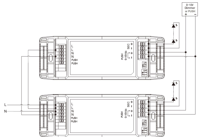
Fig. B 0-10V or Secondary PUSH
