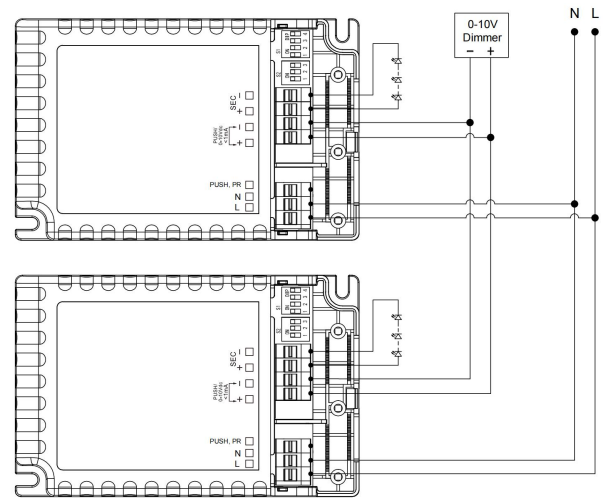
Fig. B 0-10V or Secondary PUSH
