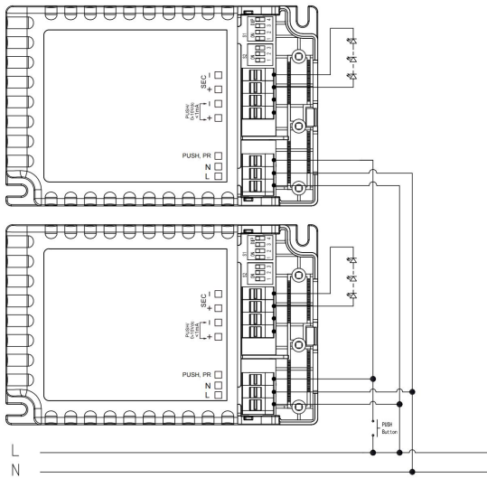
Fig. A Push Dimming OR Corridor function
