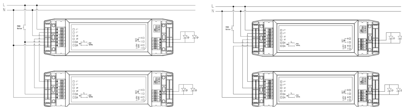
Fig. A Push Dimming
