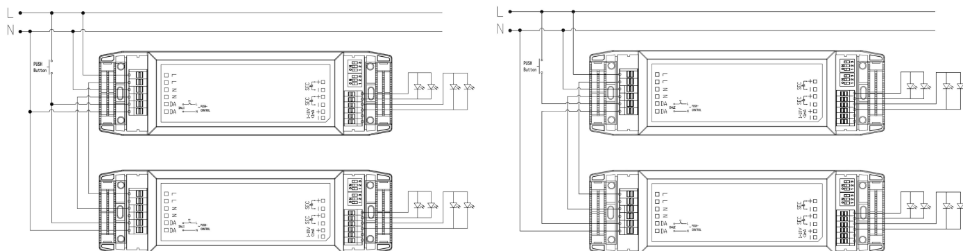
Fig. A Push Dimming
