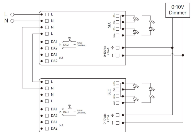
Fig. D: 0-10V Dimming
