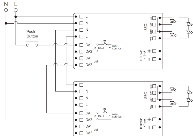
Fig. B: Push Dimming (series)
