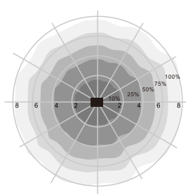
Ceiling mounting pattern (Unit: m) Suggested installation height: 2.5-15m
