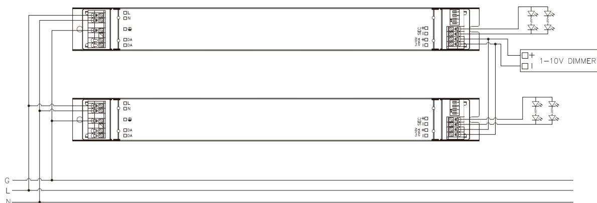
Fig.C 1-10V Dimming
