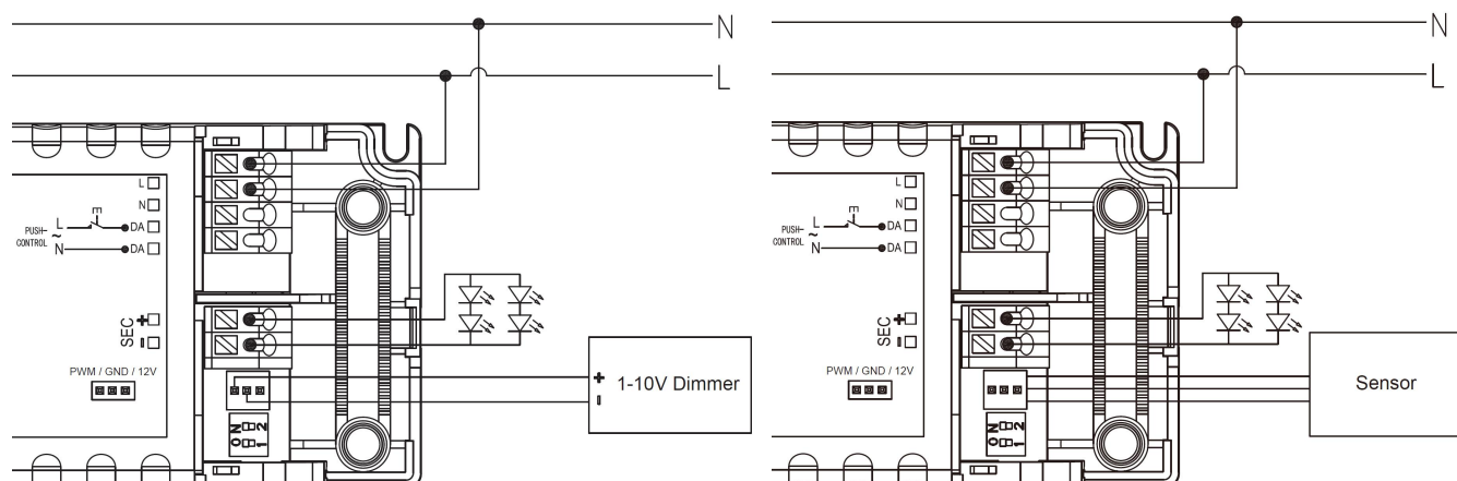
Fig. C Sensor or 1-10V Dimming
