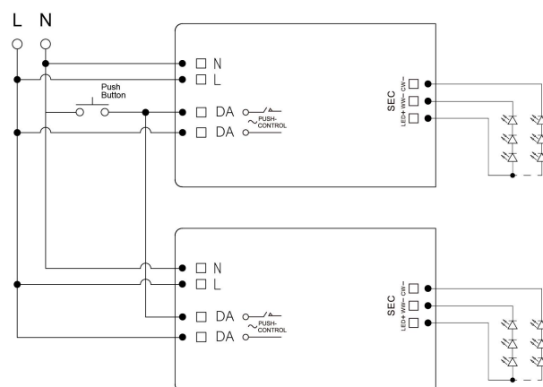
Fig. B Push Dimming
