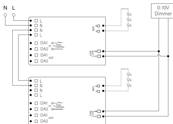
Fig. C 0-10V Dimming
