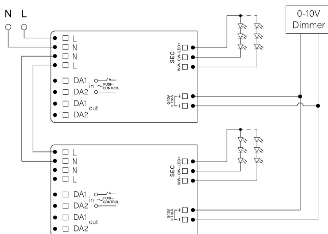
Fig. C 0-10V Dimming
