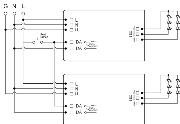
Fig. B Push Dimming
