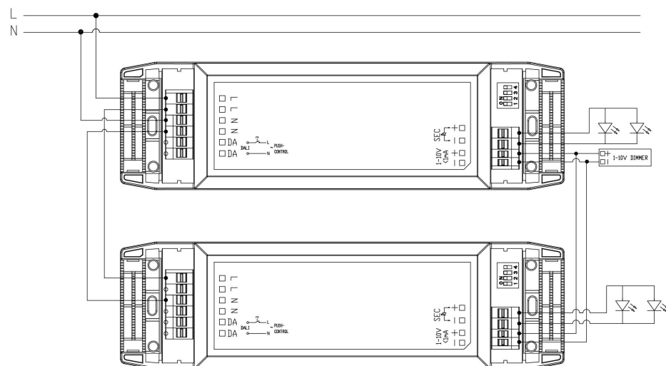
Fig. C 1-10V Dimming
