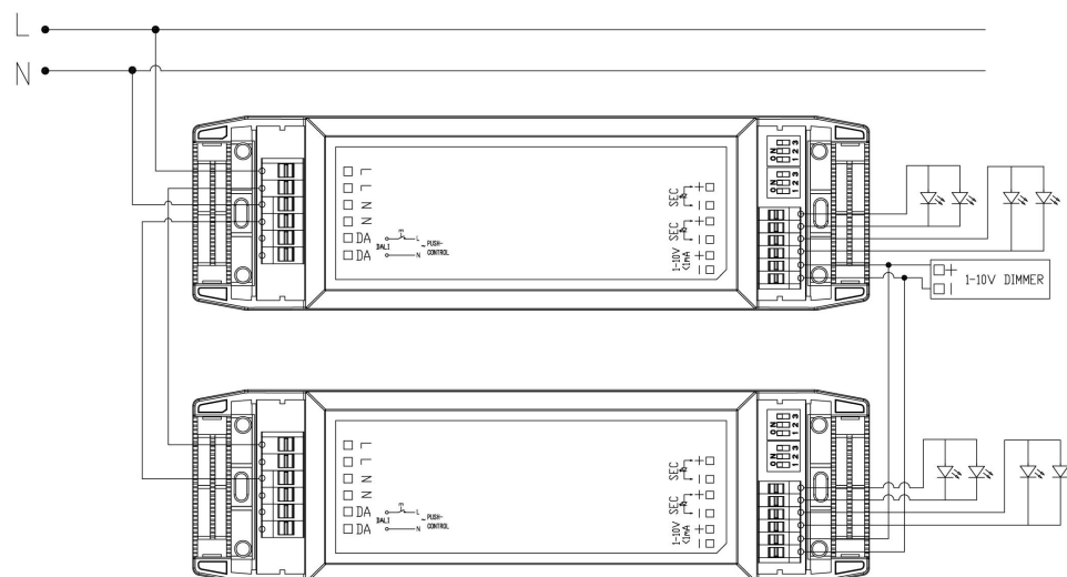
Fig. C 1-10V Dimming
