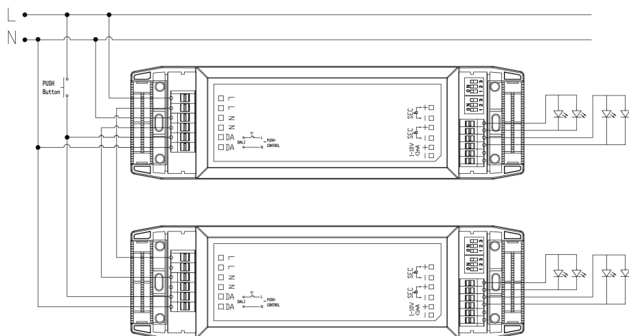
Fig. A Push Dimming
