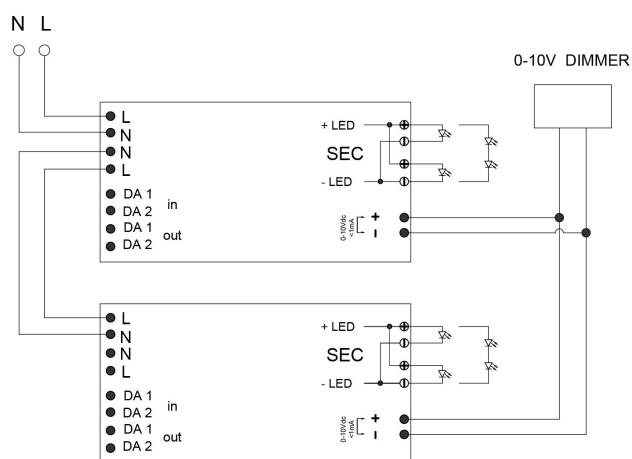
Fig.C 0-10V Dimming
