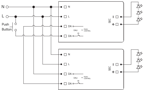
串联
