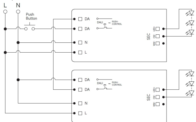
Fig. B: Push Dimming (series)
