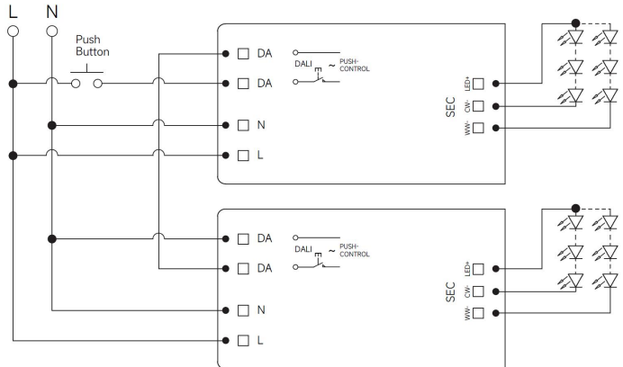
Fig. B: Push Dimming (series)
