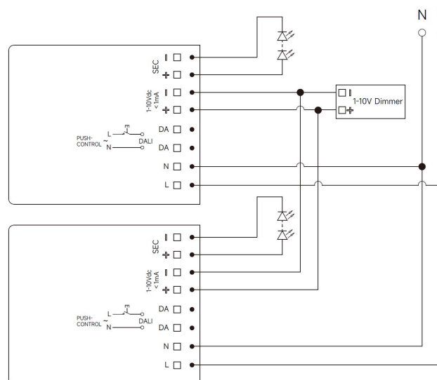
Fig. D: 1-10V Dimming
