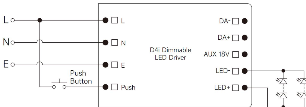
Fig. B: Push Dimming
