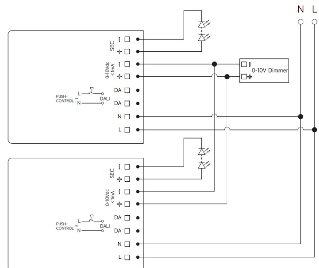
Fig. D: 0-10V Dimming
