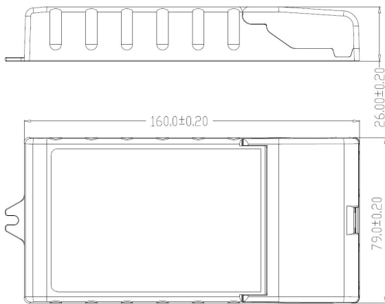
Fig.A: Independent installation
