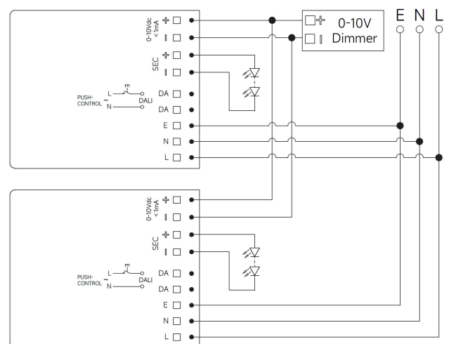
Fig. D: 0-10V Dimming
