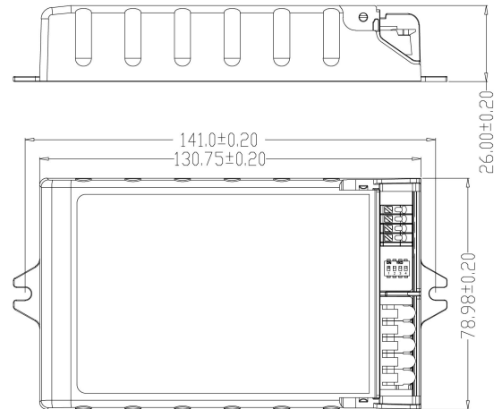
Fig.B: Built-in installation
