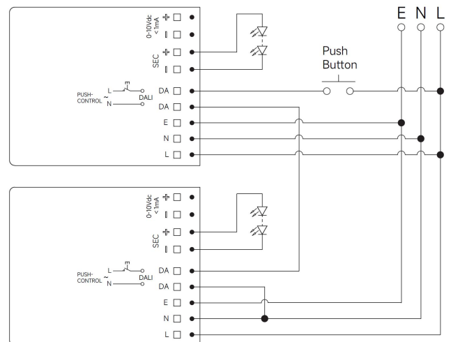
Fig. B: Push Dimming (series)
